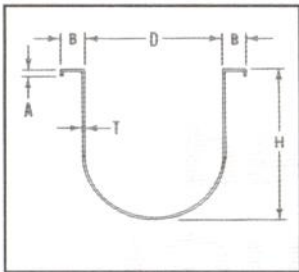
DROP OUTLET
